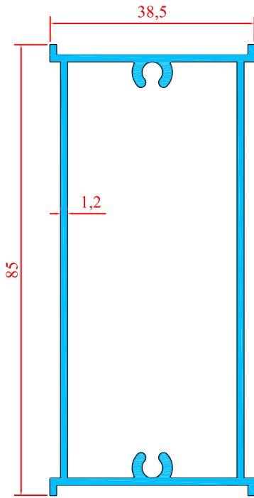
1910 0.887 Kg/m
