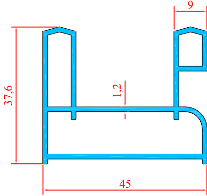
1904 0.693 Kg/m
