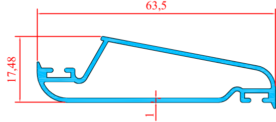
1915 0.449 Kg/m
