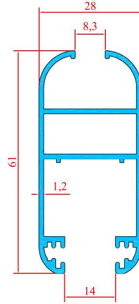
1901 0.722 Kg/m
