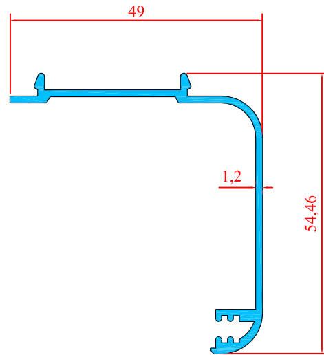
1919 0.417 Kg/m
