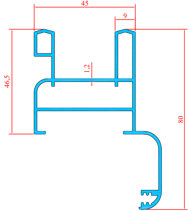
1907 0.778 Kg/m
