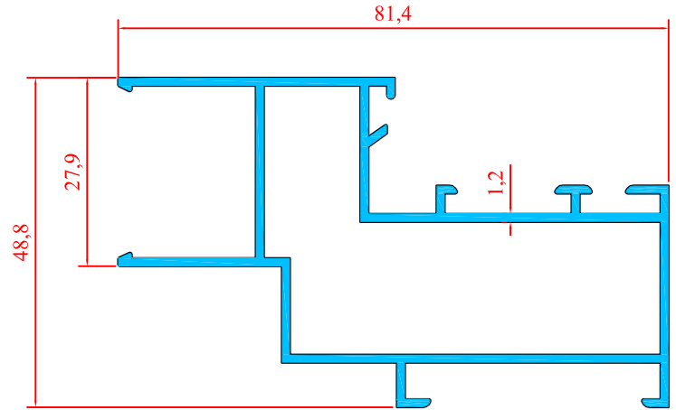
1914 0.963 Kg/m
