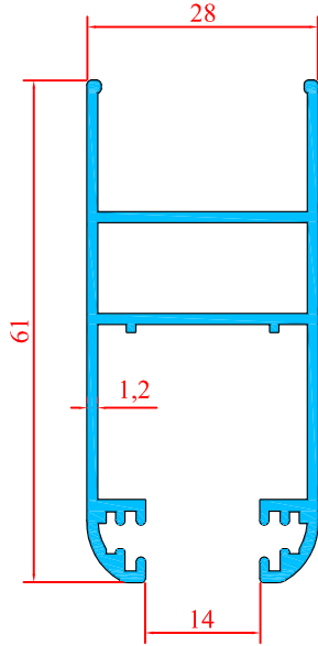
1900 0.690 Kg/m
