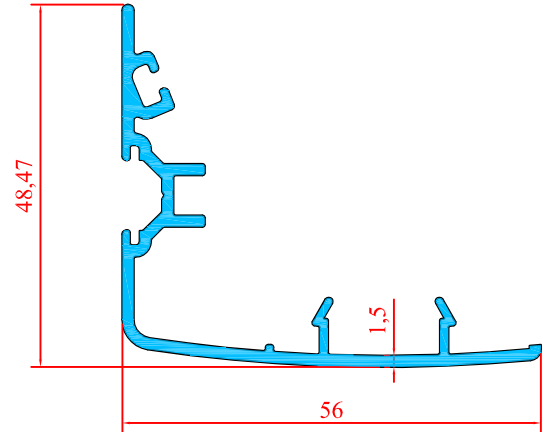
1924 0.580 Kg/m
