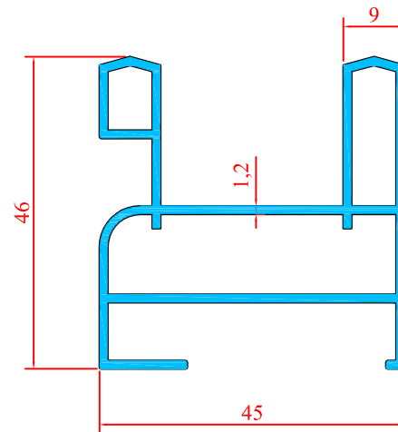
1903 0.791 Kg/m
