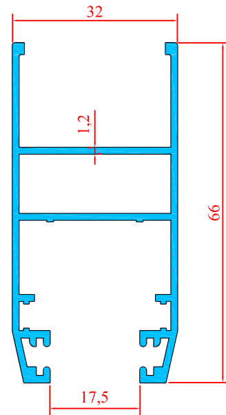
1907 0.778 Kg/m
