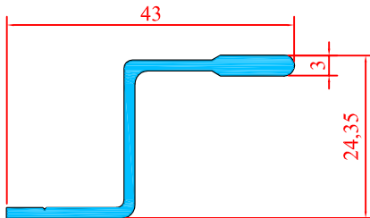
1923 0.310 Kg/m
