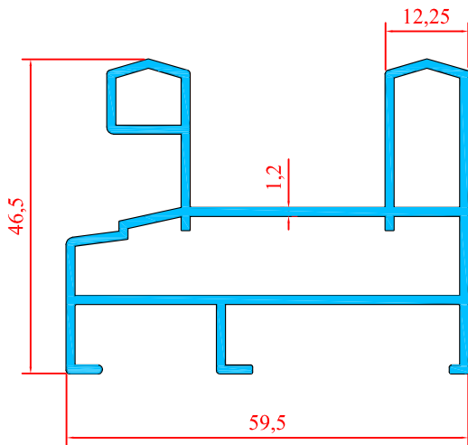
1906 0.930 Kg/m
